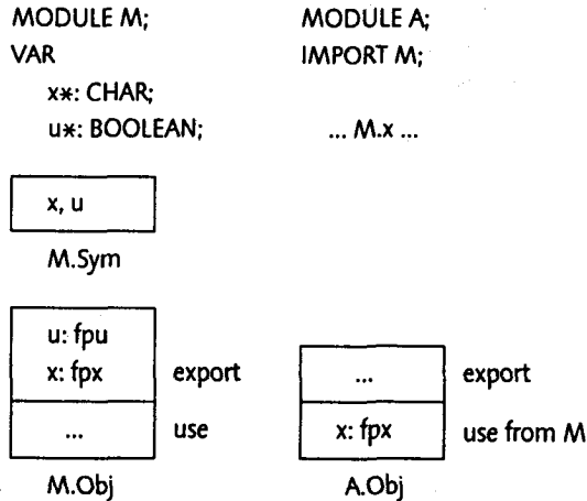
Figure 6.1 An interface M and its client A
