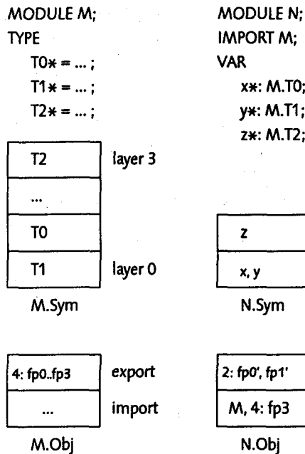
Figure 5.5 Type reexport in symbol files
