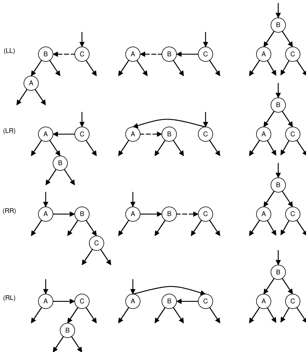
Fig. 4.49. Insertion in SBB-trees
