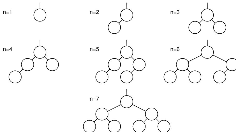
Fig. 4.22. Perfectly balanced trees
