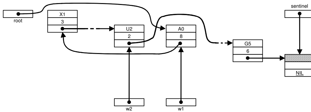
Fig. 4.12. List after re-ordering
