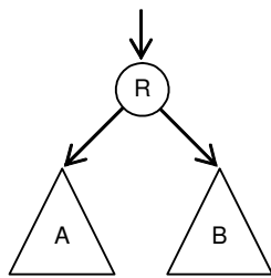
Fig. 4.24. Binary tree
