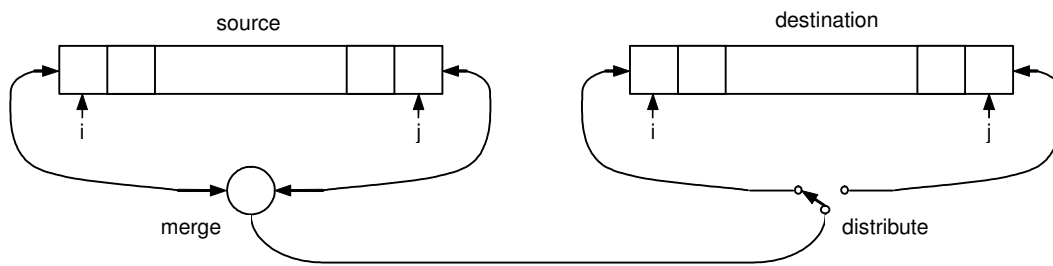
Fig. 2.12. Straight merge sort with two arrays
