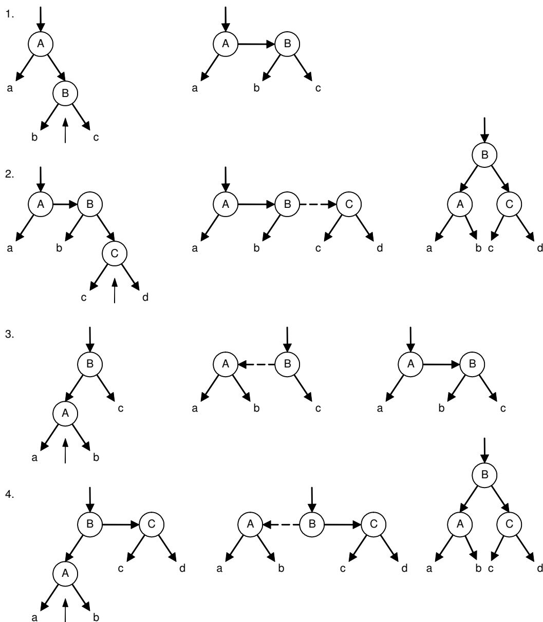
Fig. 4.48. Node insertion in BB-tree
