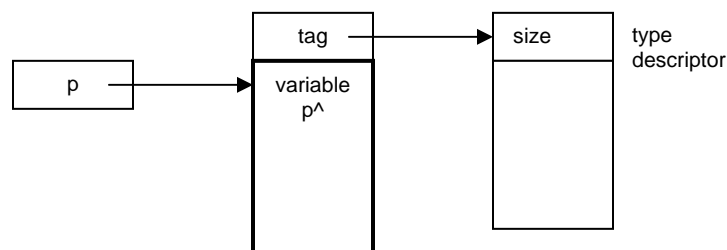
Figure 8.2 Allocation of dynamic variable p^ in the heap by procedure NEW(p)
